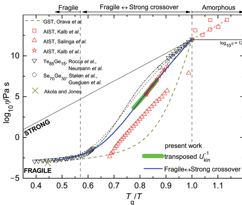
Figure 3. Angell plot for temperature dependence of viscosity. The curve for GST, from Orava et al., [7] shows the form of \eta(T) expected for a supercooled liquid of a single, high fragility ( m = 90 ). The other data shown do not fit such a form and are interpreted in terms of a fragile-to-strong crossover on cooling the liquid. For AIST, the blue line shows a generalized-MYEGA [23] fit to data in the crossover region derived from AFM-based growth-rate measurements by Kalb et al. [6] on single-film \text{Ag}_{5.5}\text{In}_{6.5}\text{Sb}_{59}\text{Te}_{27} (30 nm) and from U_{\text{kin}} data (green line) transposed from Figure 2, and to the value for \eta at 850 K derived from diffusivities in \text{Ag}_{3.5}\text{In}_{3.8}\text{Sb}_{75.0}\text{Te}_{17.7} calculated by Akola and Jones. [24] Further AIST data are those derived from reflectometry measurements by Salinga et al. [15] on sandwiched \text{Ag}_4\text{In}_3\text{Sb}_{67}\text{Te}_{26} (substrate/SiN (50 nm)/ZnS:SiO 2 (10 nm)/AIST (30 nm)/ZnS:SiO 2 (100 nm)). All these data in the crossover region show, as expected for a supercooled liquid, a stronger temperature dependence of \eta than in the amorphous or glassy state (at T_g/T > 1 showing data of Kalb et al. [22] ). The data for \text{Te}_{85}\text{Ge}_{15} are from viscosity measurements by Neumann et al. [25] and from a Kissinger analysis of conventional DSC measurements ( \Phi = 0.083\text{--}1.3 \text{ K s}^{-1} ) by Rocca et al. [26] The data for \text{Se}_{70}\text{Ge}_{30} are from viscosity values collected by Stølen et al. [27] and indentation creep measurements by Gueguen et al. [28] The dashed lines show generalized-MYEGA fits to \eta(T) for these two systems, each showing a clear fragile-to-strong crossover, which the \eta(T) for AIST resembles.
